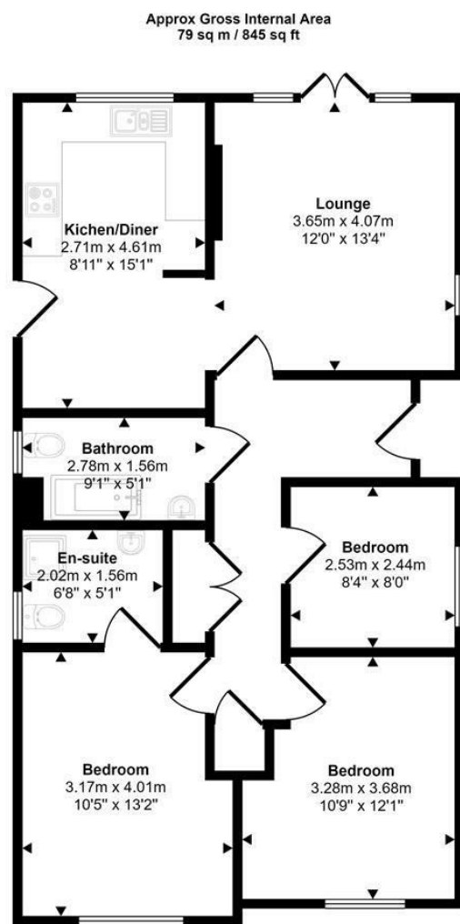
Floorplan
